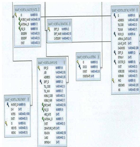
Figure 3b: Smart Hospital Schema 2
