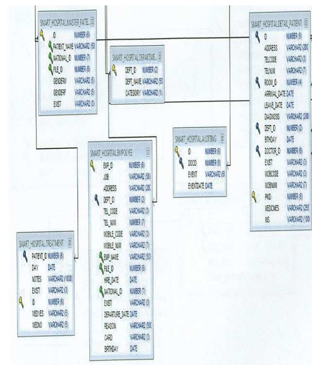
Figure 3c: Smart Hospital Schema 3
