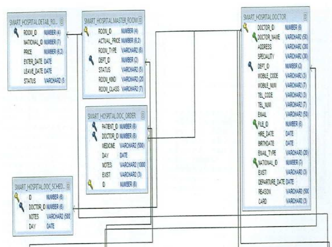
Figure 3a: Smart Hospital Schema 1
