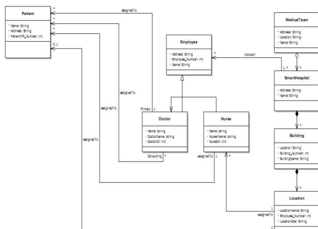
Figure 6(b): Class diagram for Asset Assignment
